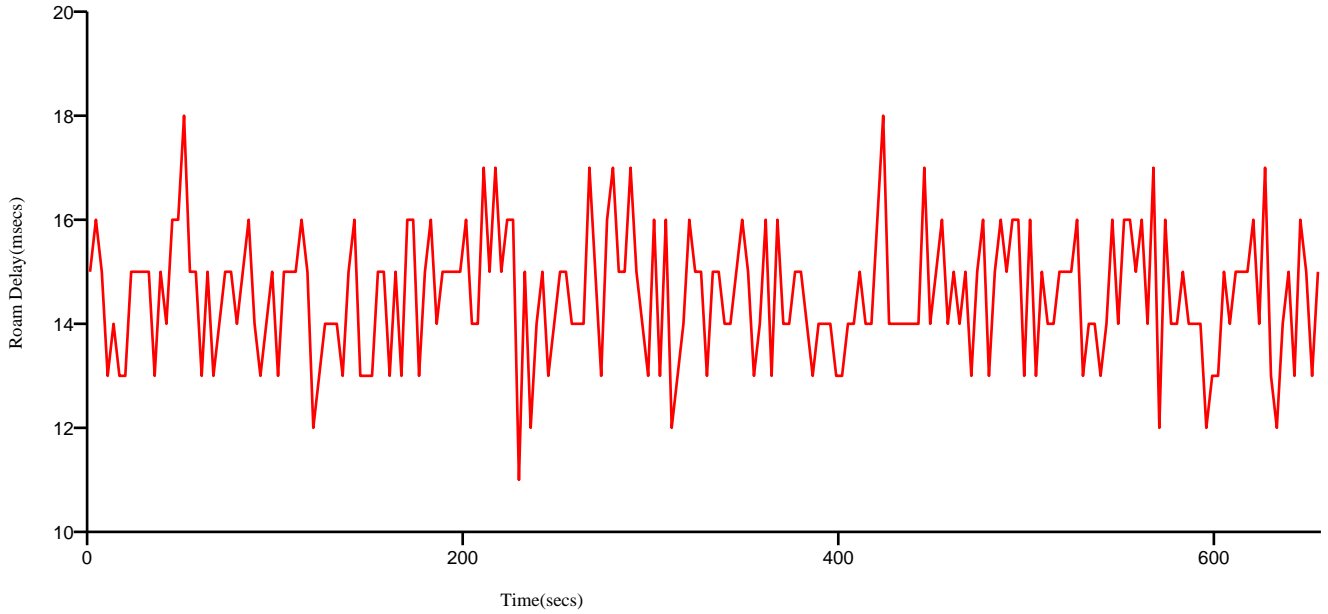
Roaming Delay Vs Time
