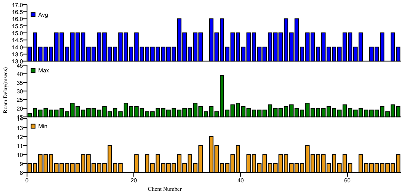
Min/Max/Average Roaming delays for Clients
